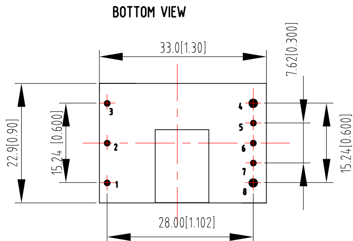
Model: AVD50B-48S05-6L
